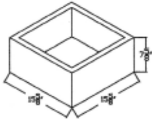
Pier Block
