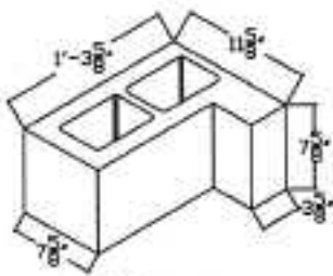
L-Corner
