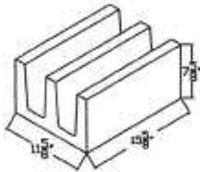
Bond Beam
