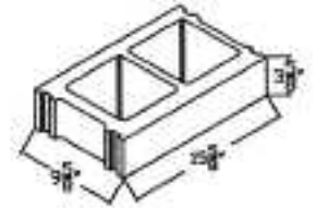
Half High
