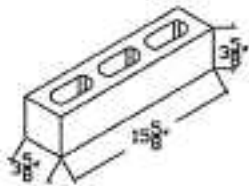
HALF HIGH
