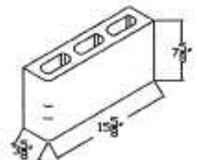
SINGLE BULLNOSE
