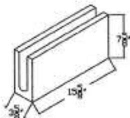
U-LINTEL
