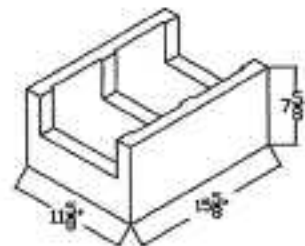
Californian Knockout
