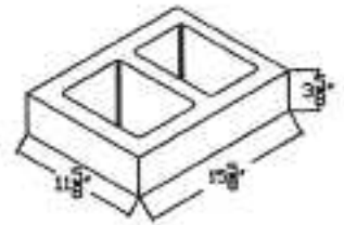
Half High
