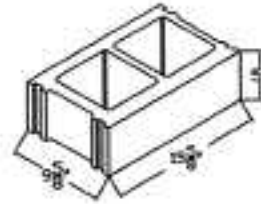
5" High (Starter)
