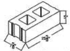
5 High (Starter)
