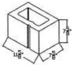
Half Block
