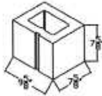
Half Block
