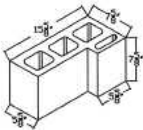
L-CORNER
