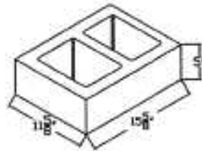
5 High (Starter)
