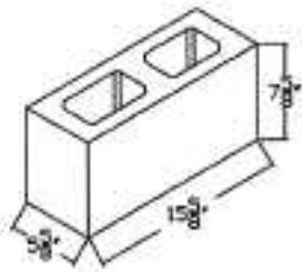
REGULAR
