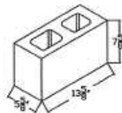
14" CORNER
