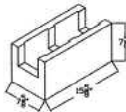
Californian Knockout
