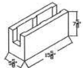
CALIFORNIAN KNOCKOUT
