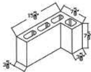
L-CORNER
