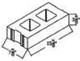
Half High
