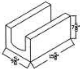
Bond Beam
