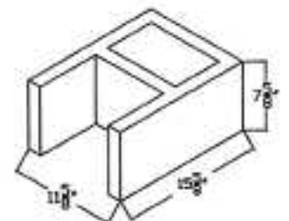
End Out
